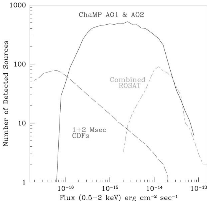
Fig. 2. Number of sources predicted from the ChaMP survey (for 137 ChaMP fields from Chandra Cycle 1 and Cycle 2) compared to numbers of sources from the Chandra Deep Fields and the ROSAT surveys analyzed by T. Miyaji, G. Hasinger, & M. Schmidt, 2000, A&A , 353, 25. An impressive \approx 6000 ChaMP sources are expected in total, and these largely lie at intermediate 0.5–2 keV flux levels of (4\text{--}60)\times 10^{-16} erg cm ^{-2} s ^{-1} . From [35]
