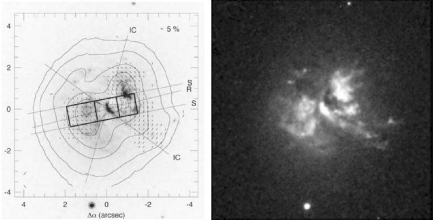
Fig. 8. The powerful radio galaxy Cygnus A . The image on the right is a combination of B, V, R and I broad band and [O III] and H \alpha narrow band exposures from the HST WFPC 2 archive with the addition of a B-band exposure with Keck. The B-band contour map on the left is from the Keck LRISp polarimeter showing the measured E -vectors and the location of the apertures used for spectropolarimetry (a negative version of the colour image is shown as an underlay). The position of the radio axis (R) and the outline of the ionization cone (IC) are shown. The equatorial ring on the southeast side consists of starlight and is unpolarized
