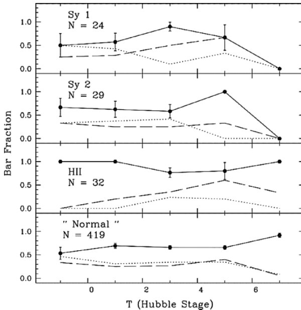
Fig. 9. Relation between large-scale bars and nuclear starburst/AGN: The fraction of barred galaxies as a function of Hubble type and nuclear types is shown for the extended 12 \mu\text{m} Galaxy Sample. Nuclear types (HII, Sy 1, Sy 2, LINER) are taken from NED. Quiescent nuclei without any of these signatures are denoted as “normal”. Optically-based RC3 bar classes are shown as dotted lines (unbarred), dashed lines (weakly barred SAB), and solid lines (weakly and strongly barred SAB+SB). The data bins are as in Fig. 3. Numbers under the panel label give the number of galaxies in each subsample. (Figure is from Hunt & Malkan 1999)
