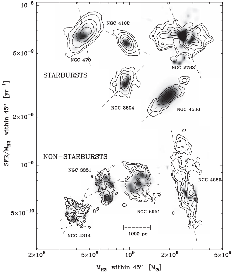
Fig. 6. High resolution ( 2'' or 100–200 pc) observations of molecular gas and star formation in the inner few kpc of barred galaxies: CO (1–0) intensity (contours) maps of the circumnuclear region of barred galaxies are overlaid on 1.5 or 4.9 GHz radio continuum map or H\alpha map (greyscale). The dotted line is the P.A. of the large-scale stellar bar/oval. A wide range in gas distributions and in SFR per unit mass of molecular gas ( SFR/M_{H_2} ) is present. Systems with high/low circumnuclear SFR/M_{H_2} are denoted as starbursts/non-starbursts. Part of the range in SFR/M_{H_2} and the variety of gas distributions can be understood in terms of different stages of bar-driven inflow and the critical density for the onset of SF. (From Jogee et al. 2004c; see text for details)
