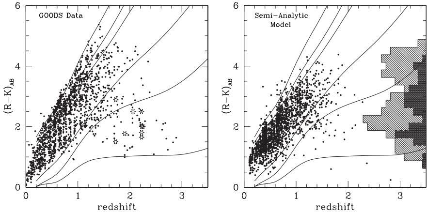
Fig. 2. Observed (R-K)_{AB} colour vs redshift for the GOODS CDFS [left] and the semi-analytic mock catalog [right]. Tracks are shown for single age, stellar metallicity populations with ages of 13.5, 5.8, 3.2, 1, 0.5, and 0.1 Gyr (unreddened), from top to bottom . The color distribution of galaxies with K < 22 in the redshift range 1.7 < z < 2.5 is shown in the right panel as histograms (diagonal hatched: GOODS ; horizontal fill: mock catalog). Taken from [43] (Reproduced by permission of the AAS)
